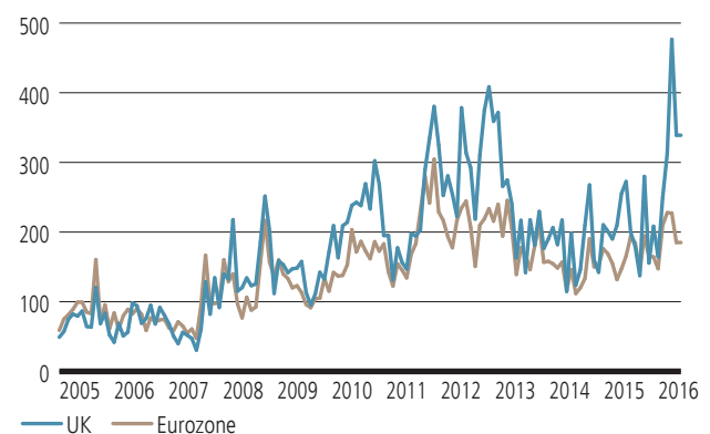
Chart 1: Certainly uncertain
